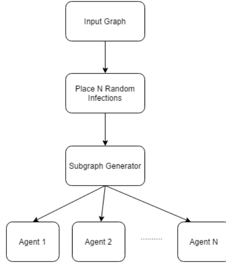
Figure 4.1: Generating agents
